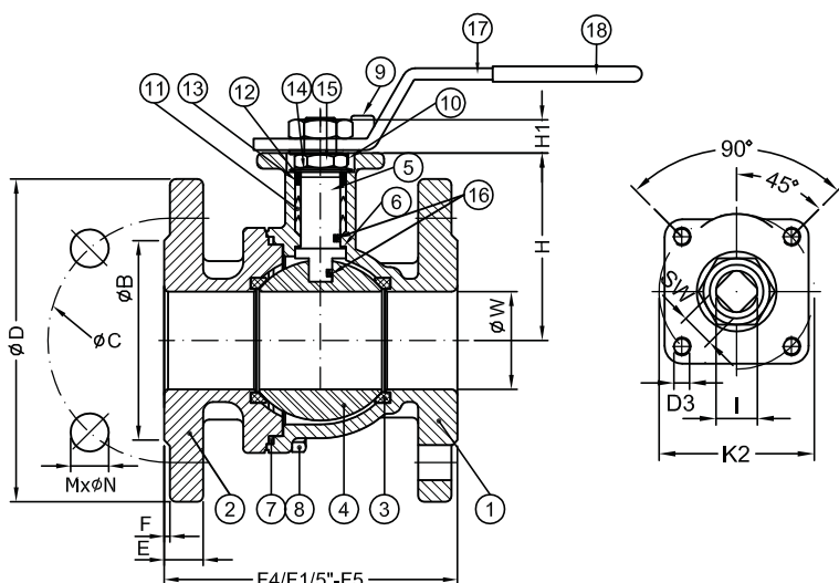
BODY DIMENSIONS(mm)
